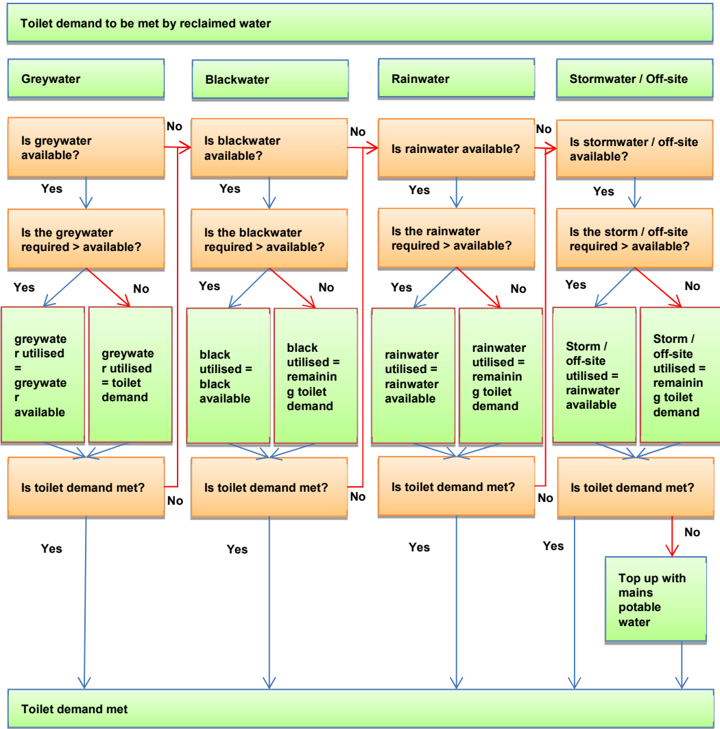
Figure 7 Flowchart showing the reclaimed water utilisation methodology
