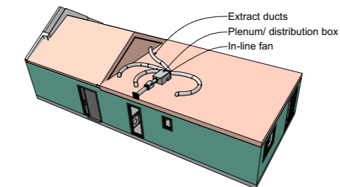
Ventilation system
