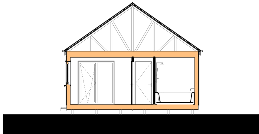
SHORT SECTION 02
