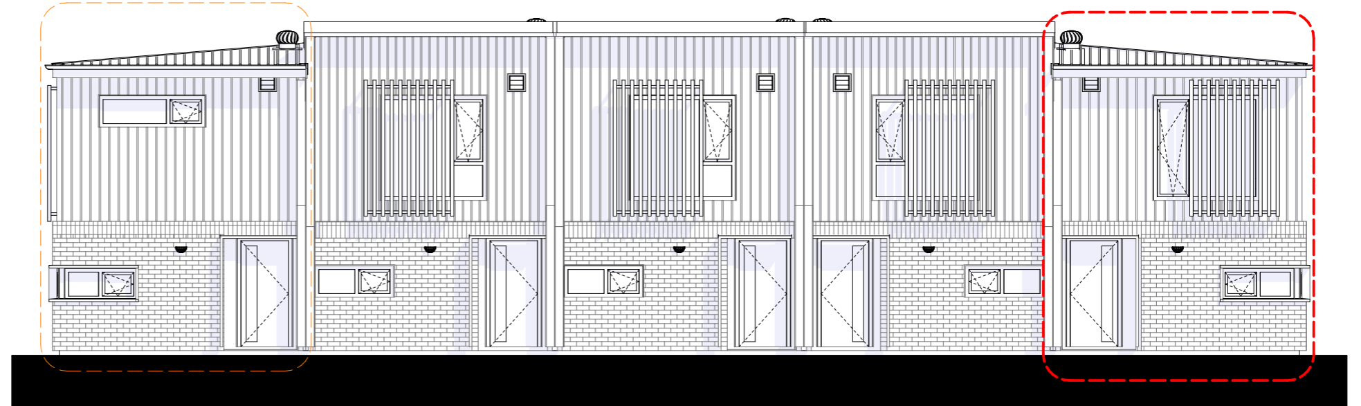
WEST ELEVATION
