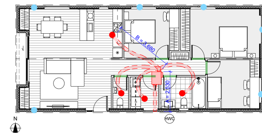
Worked ventilation plan
