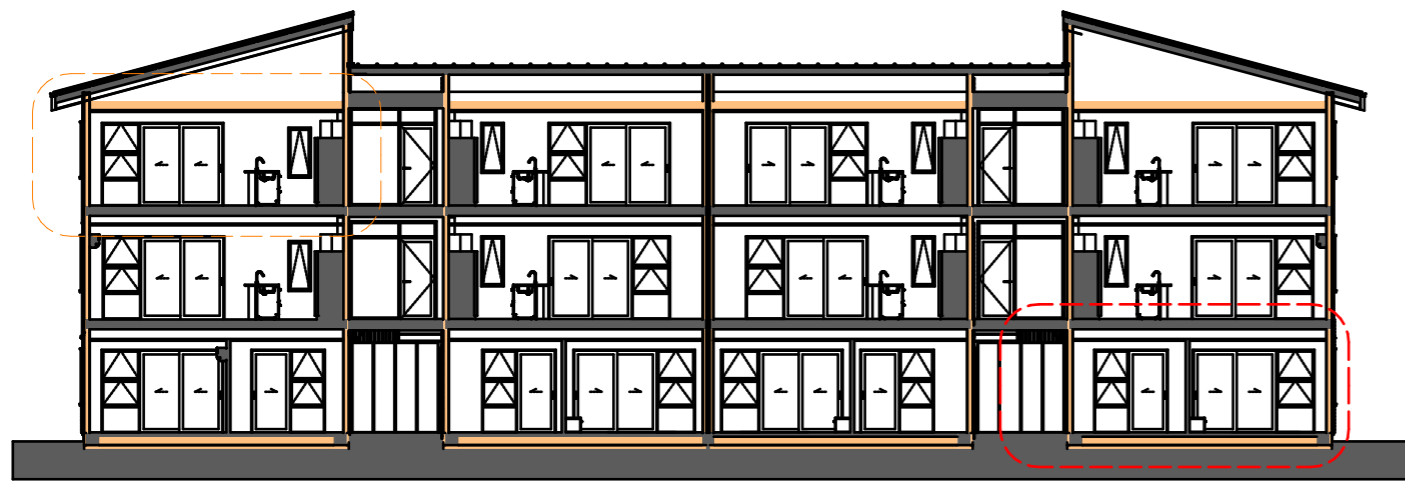
SECTION A
