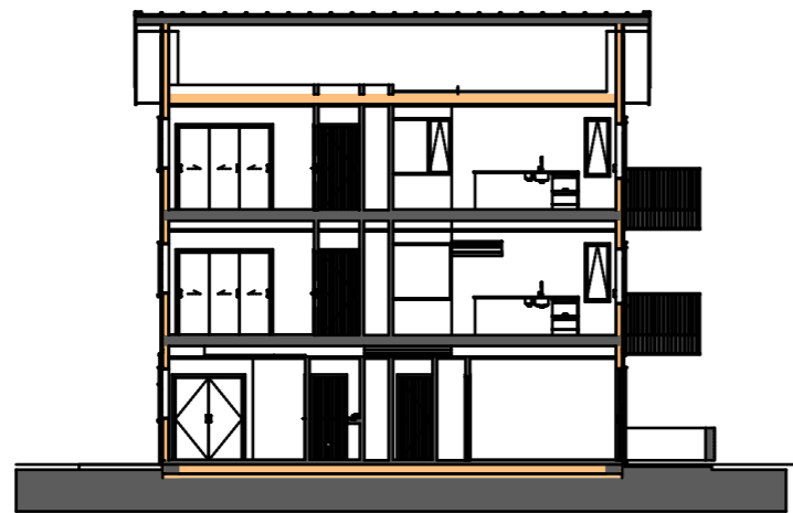
SECTION B
